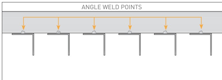
TOP ELEVATION DETAIL OF 40 X 40MM STYLE
