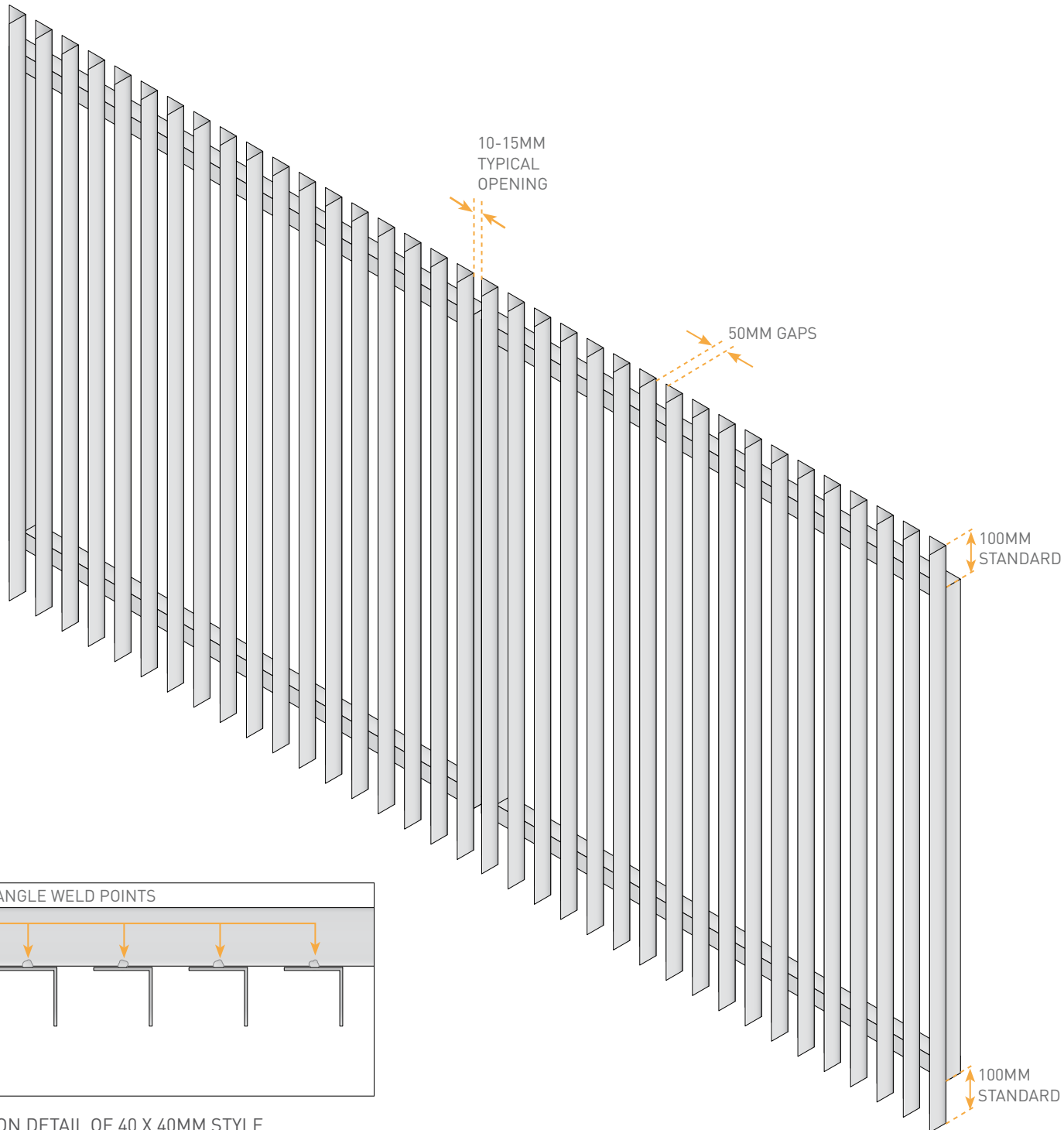
TOP ELEVATION DETAIL OF 40 X 40MM STYLE
